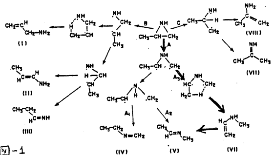
The possible ways of ring-opening in propyleneimine and the possible products of chemical formula of C 3 H 7 N.
