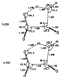
FIG. 1. Optimized geometries for the 5-center transition state. Bond distances are in Å and angles in degrees. All structures are planar.
