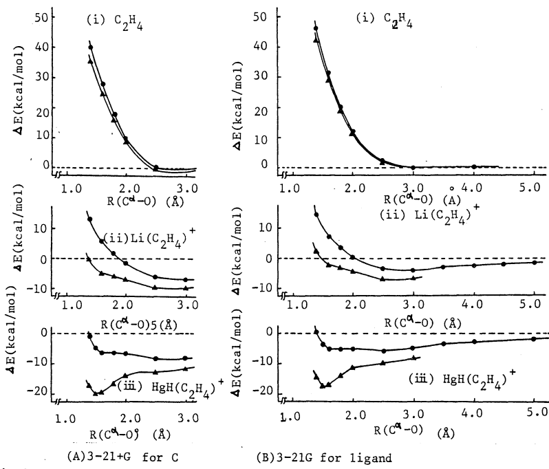
Fig.1 Total energy changes caused by approaching of nucleophile
