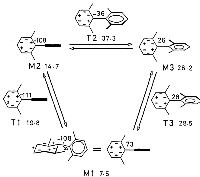
1-(2',b'-Dimethylphenyl)-(2S,bR)-2,b-dimethylcyclohexane
