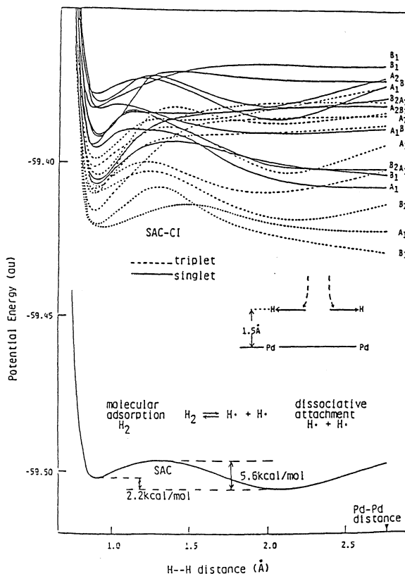
Figure 7. Potential energy curves of the ground and excited states of the \text{Pd}_2\text{-H}_2 system as a function of the \text{H-H} distance of the \text{H}_2 molecule at 1.5\text{\AA} apart from the \text{Pd}_2 fragment. (SAC and SAC-CI methods)
