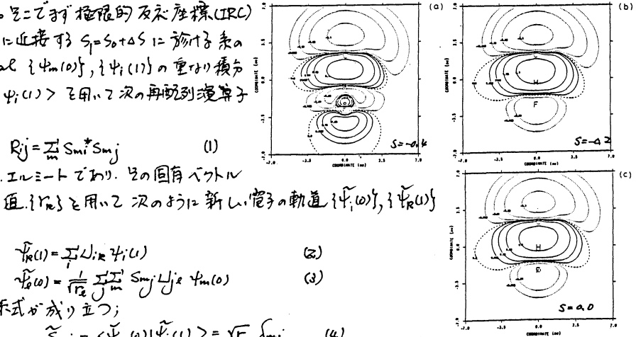
図1. IRC上の \tilde{\psi}_i
