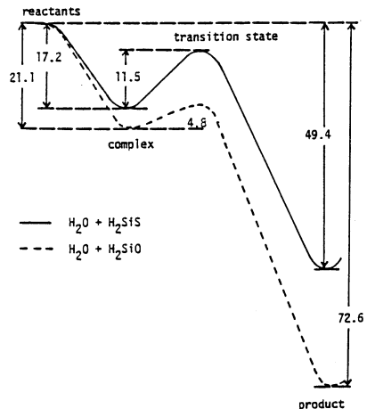
図6 MP3/6-31G**/16-31G 値 (kcal/mol)
