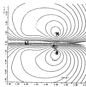
Fig. 6 CONTOUR PLOTS OF NATURAL ORBITAL DENSITY, \psi_{1b_1} OF THE {}^2B_2 STATE OF LI-H _2 . UNITS: hartree/bohr ^3 .
