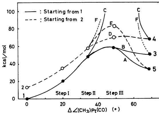
Fig. 4 Energy change in the CO insertion
