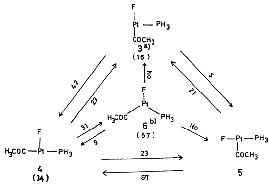
Fig.3 Relative stabilities of several Pt(COCH_3)F(PH_3) and potential barrier of the mutual isomerization among them. in parentheses; the relative energy (kcal/mol), number near arrow; the potential barrier (kcal/mol)
