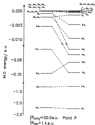
Fig. 5 Orbital energies in the lowest {}^2B_2 state.
