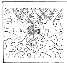
図7. Deformation Density of trans-[η-C 5 H 5 ]Fe(CO) 2
